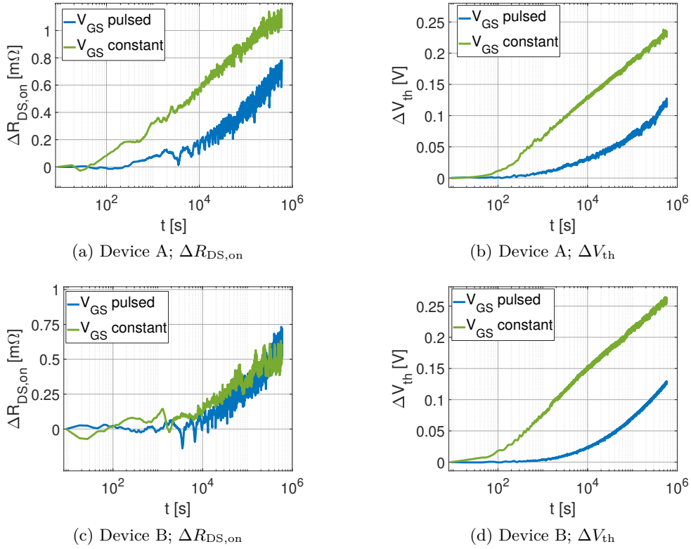
Figure 3.52: Results device A and device B; T_{vj} = 150\text{ }^{\circ}\text{C}
