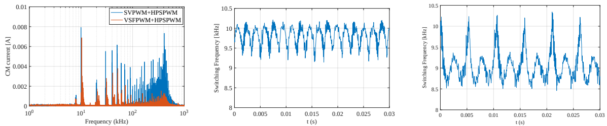
Figure 3.19: Measured CM current in frequency domain (left) and switching frequency applying VFS-PWM in SV-PWM (mid) and HPS-PWM (right) modulated EDS.
