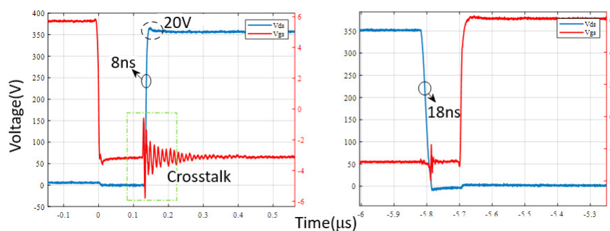
Figure 3.54: Waveforms captured in a power section with discrete GaN HEMTs
