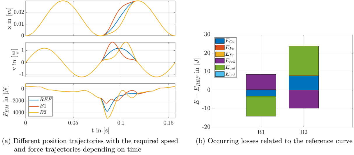
Figure 3.6: Investigations for a Trajectory Variation to Improve the Energy Conversion for a Four-Stroke Free-Piston Engine
